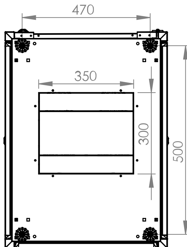
Bottom view
