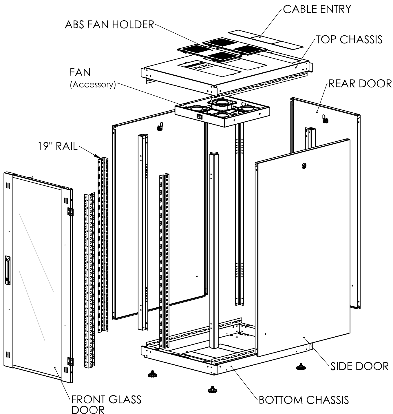
Exploded view
