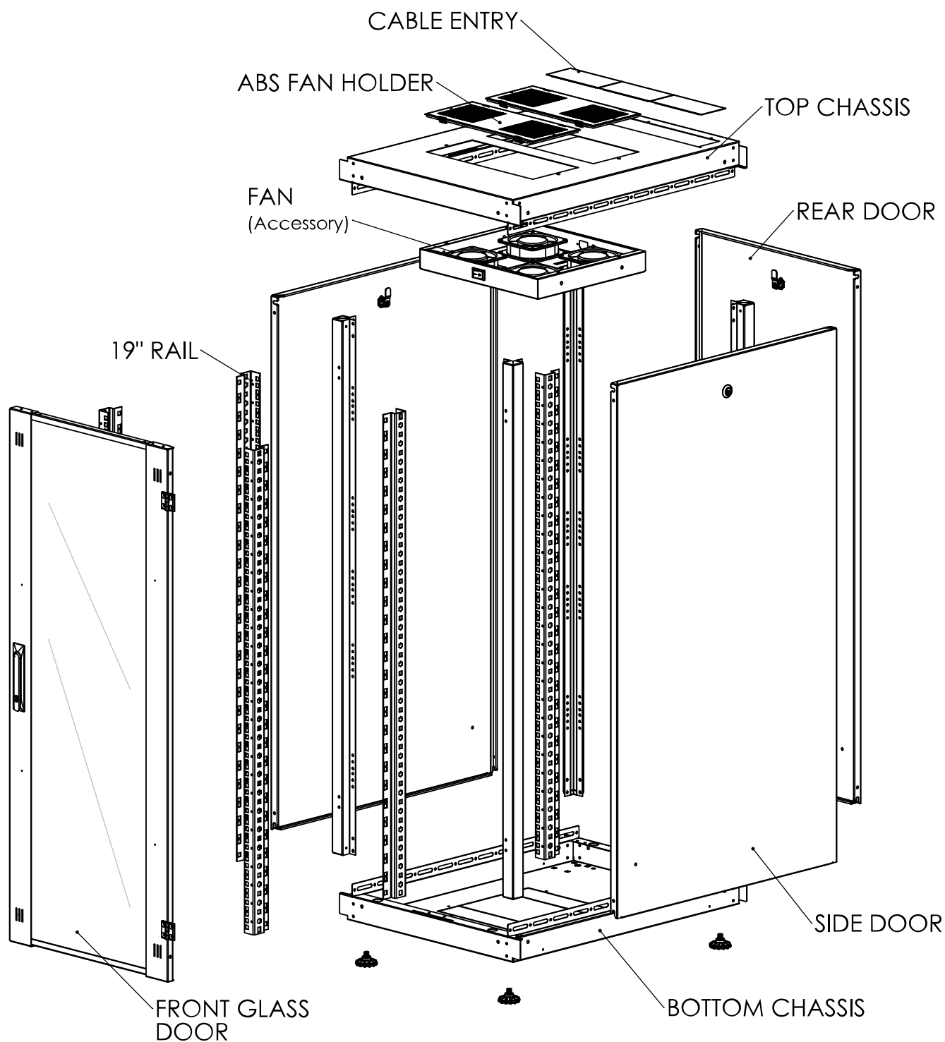
Exploded view
