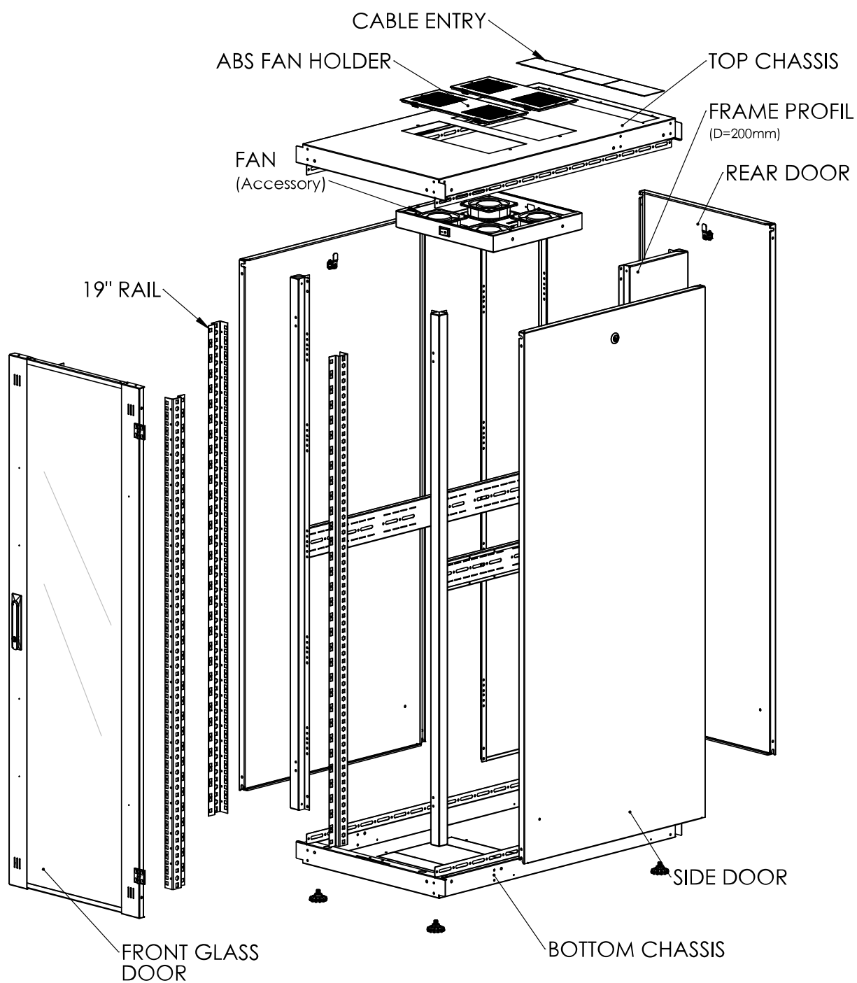
Exploded view
