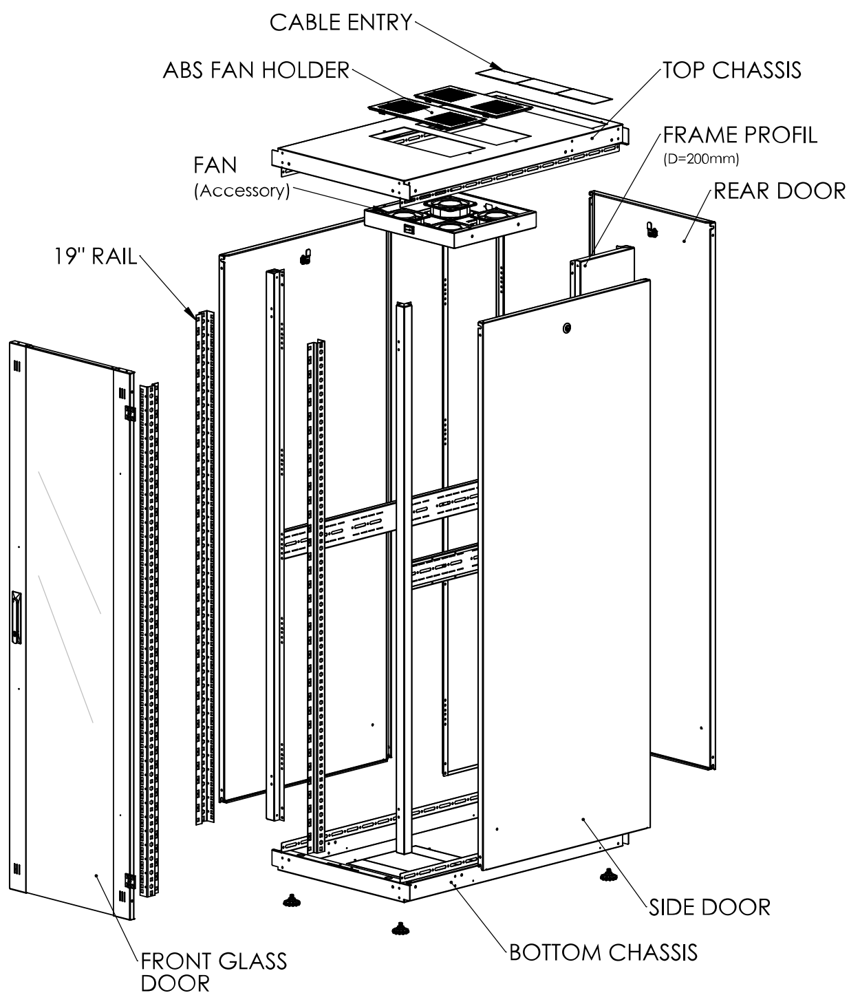
Exploded view
