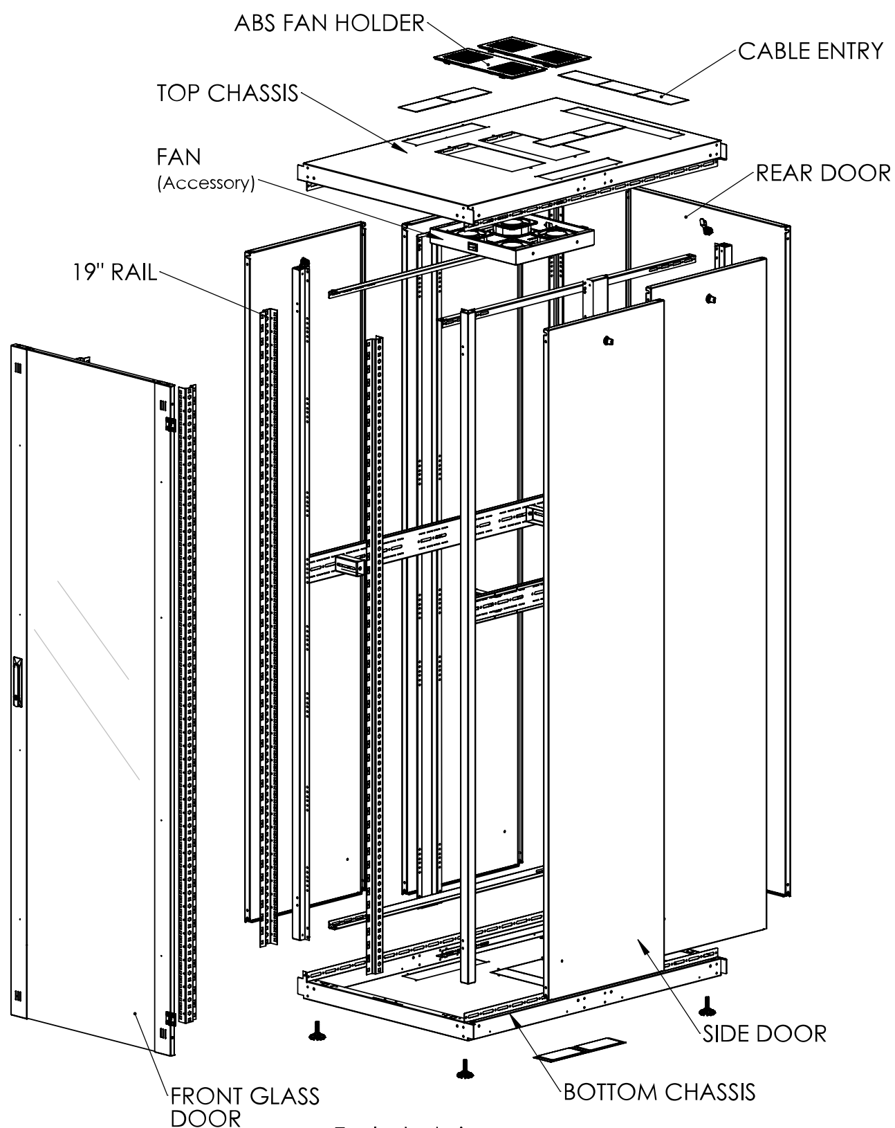
Exploded view
